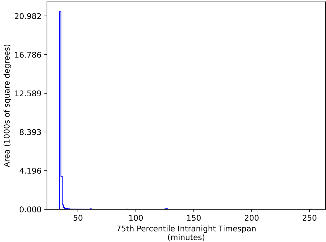
too_elab_r32_d2_gz_v3.4_10yrs All sky gr bands: 75th Percentile Intranight Timespan
