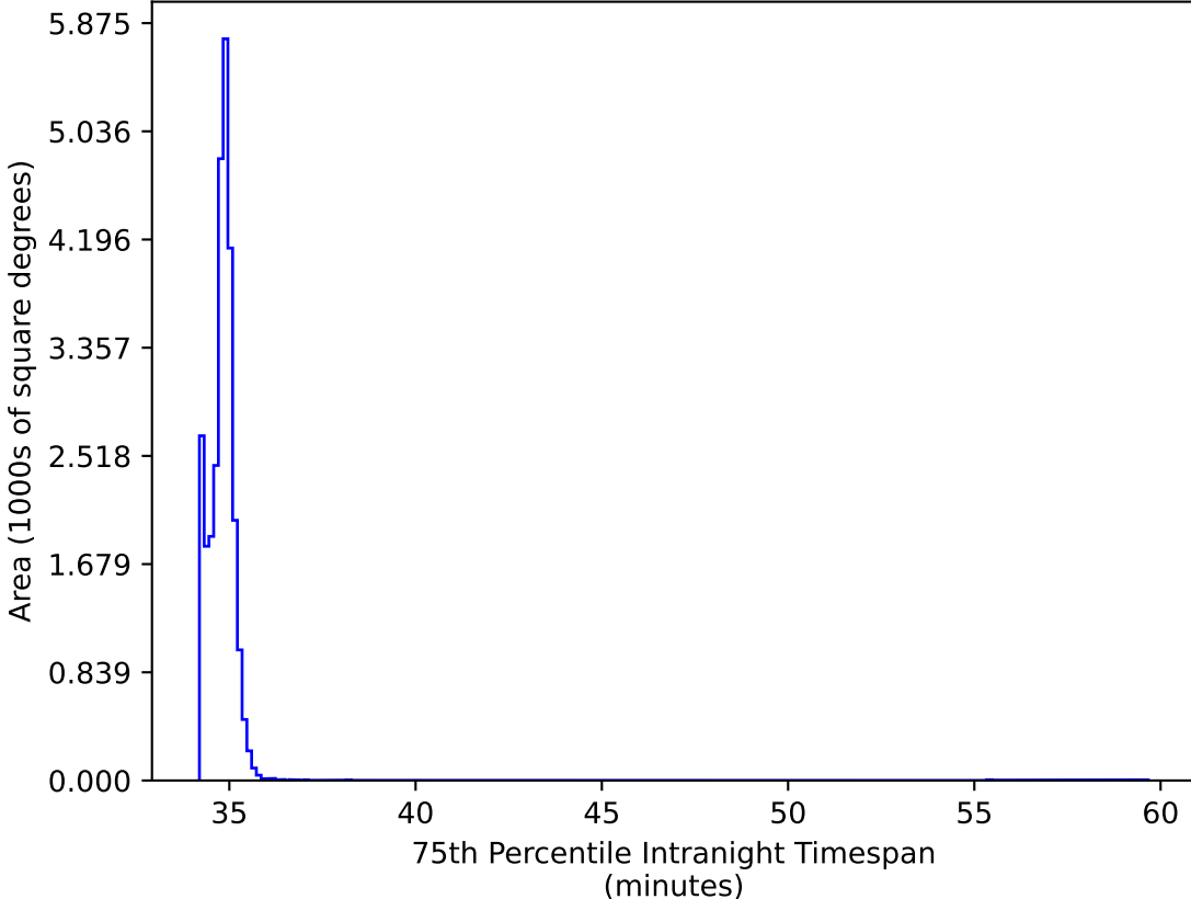
too_elab_r32_d2_gz_v3.4_10yrs All sky all bands: 75th Percentile Intranight Timespan
