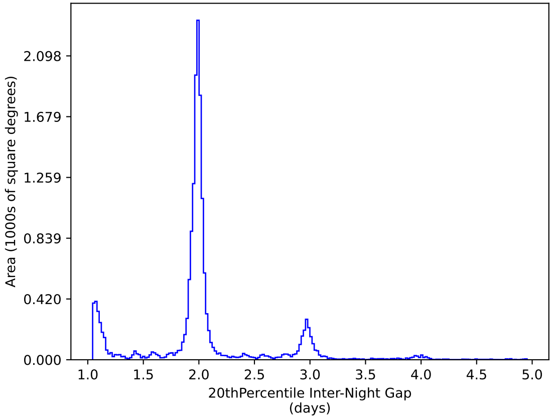
too_elab_r32_d2_gz_v3.4_10yrs WFD y band: 20thPercentile Inter-Night Gap
