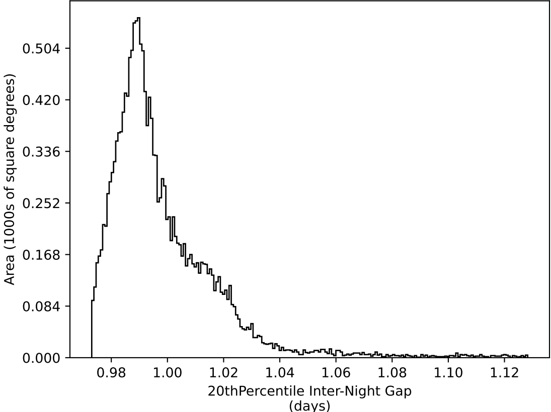
too_elab_r32_d2_gz_v3.4_10yrs WFD all bands: 20thPercentile Inter-Night Gap
