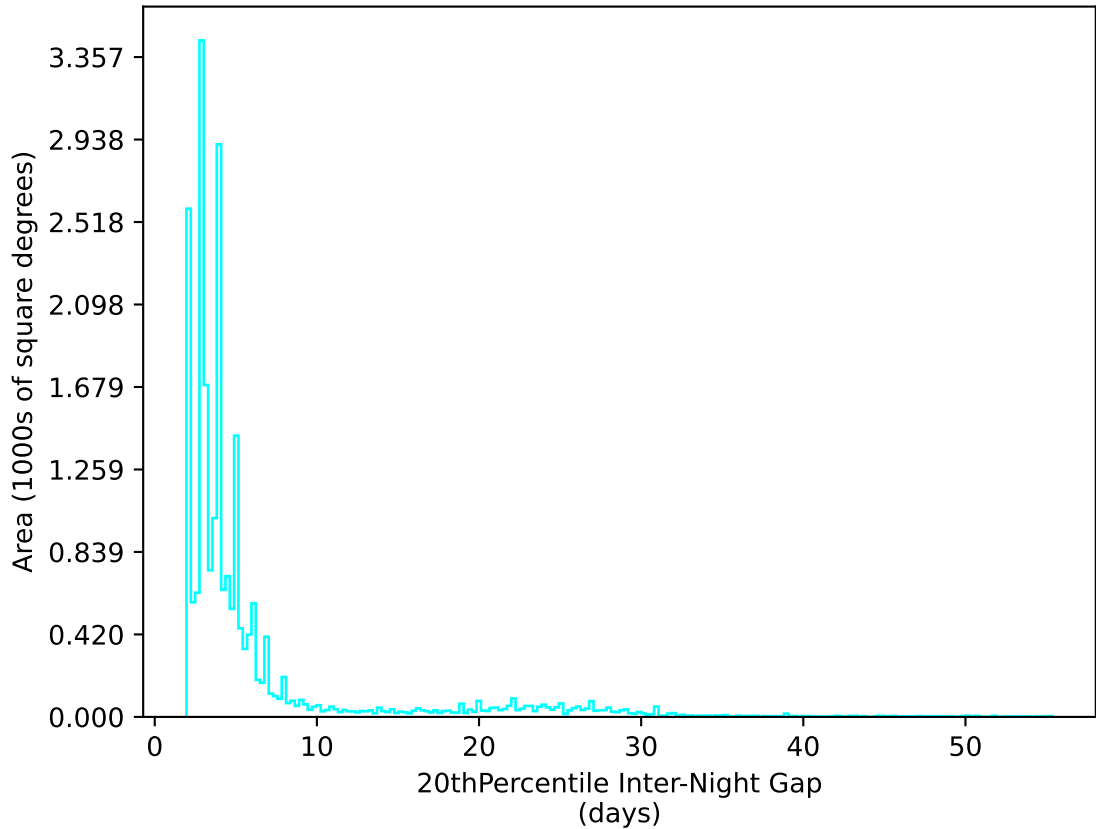
too_elab_r32_d2_gz_v3.4_10yrs All sky u band: 20thPercentile Inter-Night Gap
