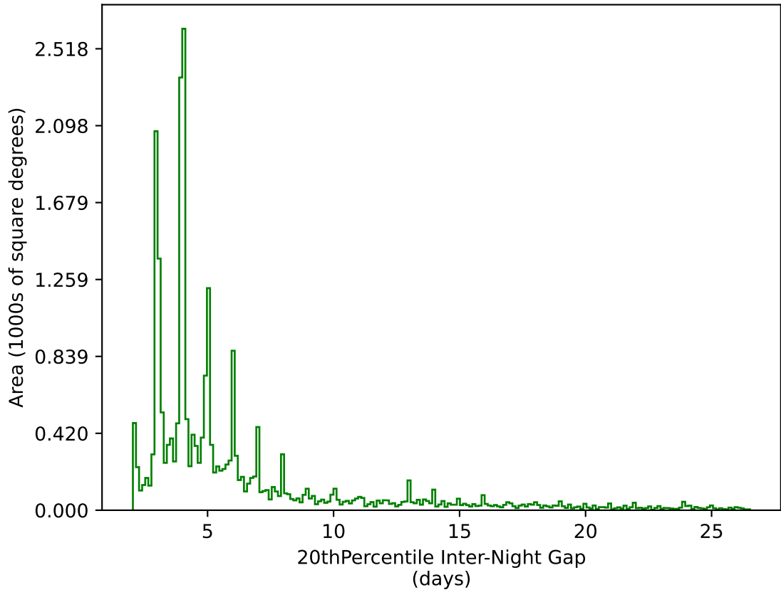
too_elab_r32_d2_gz_v3.4_10yrs All sky g band: 20thPercentile Inter-Night Gap
