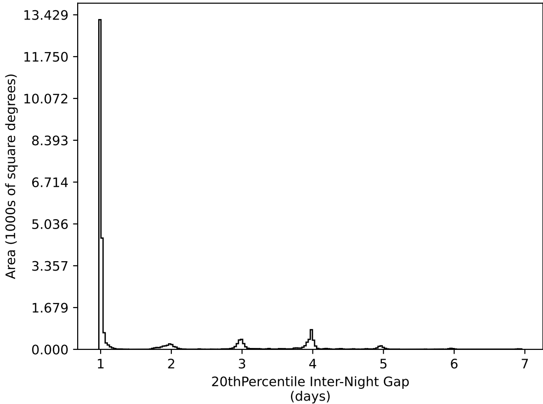
too_elab_r32_d2_gz_v3.4_10yrs All sky all bands: 20thPercentile Inter-Night Gap
