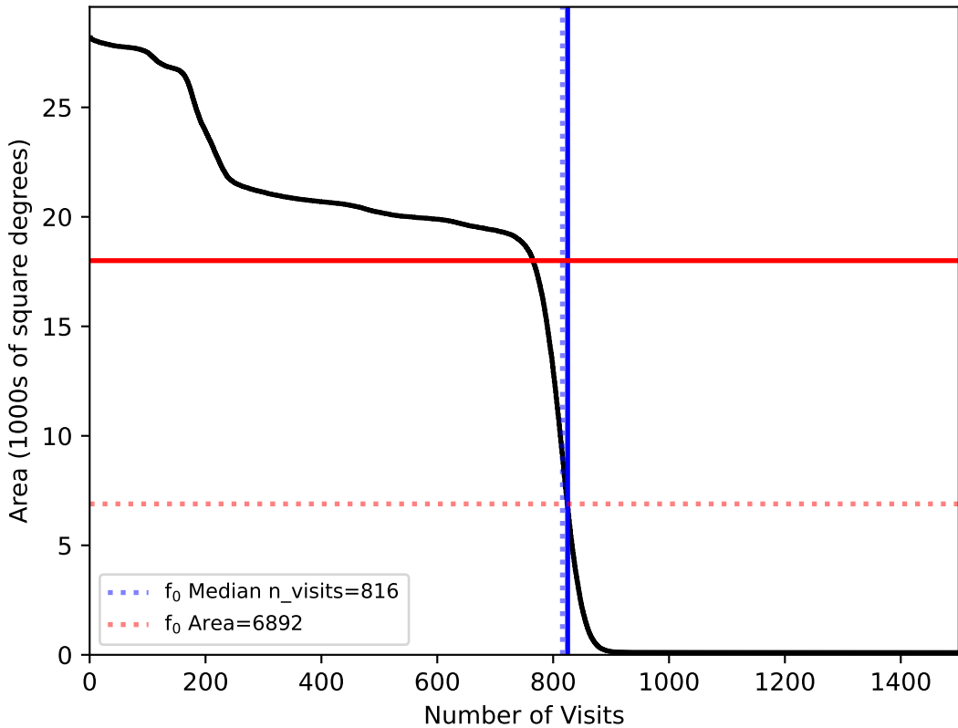
too_elab_r32_d2_gz_v3.4_10yrs : f0
