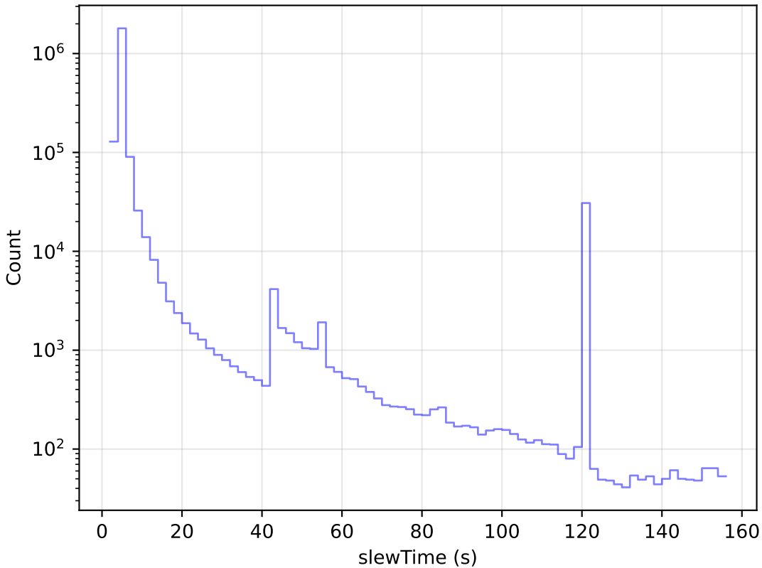
too_elab_r32_d2_gz_v3.4_10yrs All visits: Slew Time Histogram
