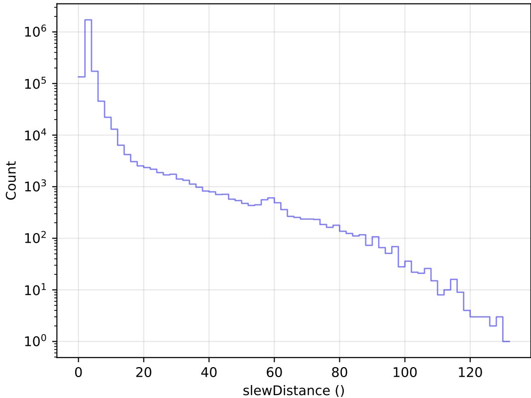
too_elab_r32_d2_gz_v3.4_10yrs All visits: Slew Distance Histogram
