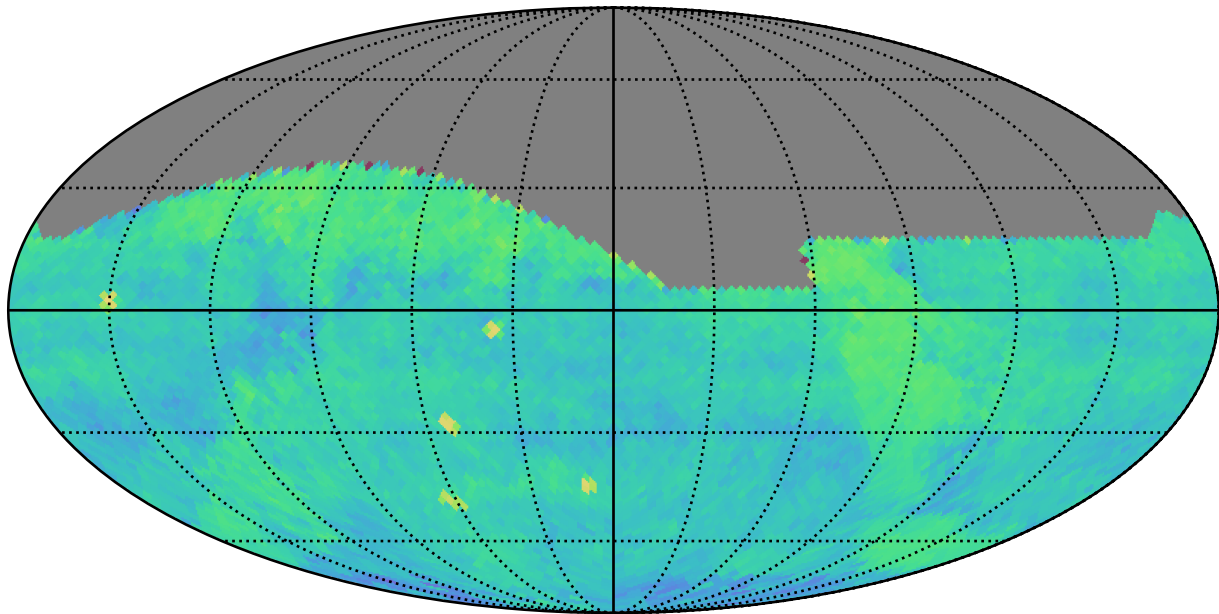
too_elab_r32_d2_gz_v3.4_10yrs (g or r or i): PairFraction
