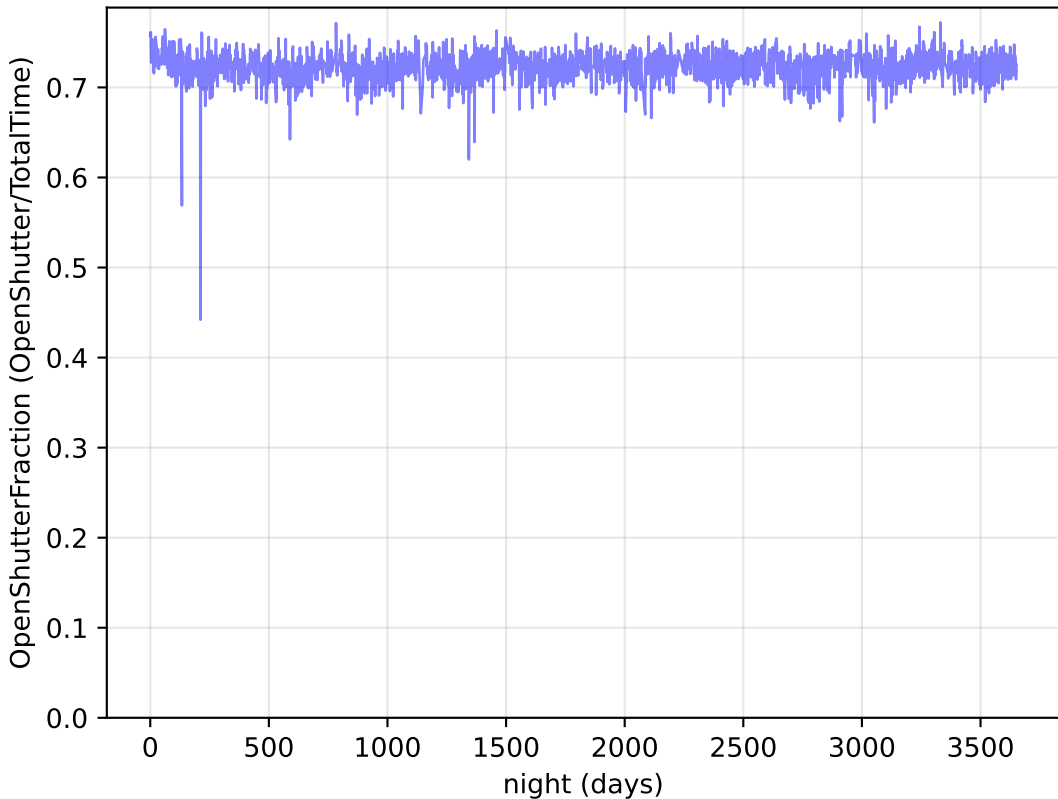
too_elab_r32_d2_gz_v3.4_10yrs : OpenShutterFraction
