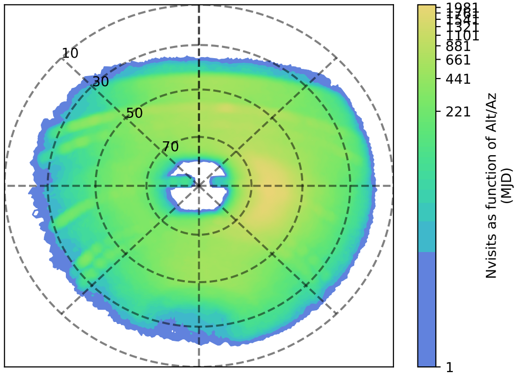
too_elab_r32_d2_gz_v3.4_10yrs y: Nvisits as function of Alt/Az
