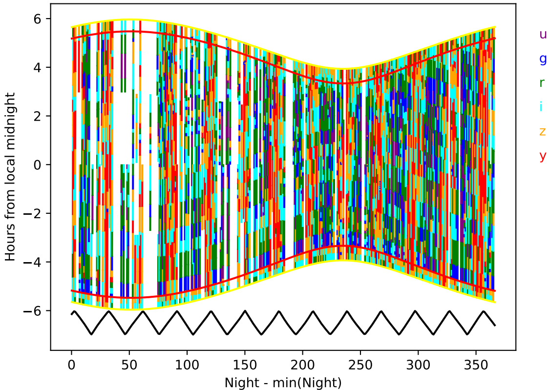
too_elab_r32_d2_gz_v3.4_10yrs year 9-10: Hourglass
