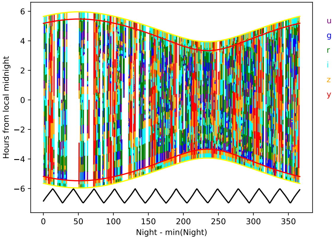
too_elab_r32_d2_gz_v3.4_10yrs year 8-9: Hourglass
