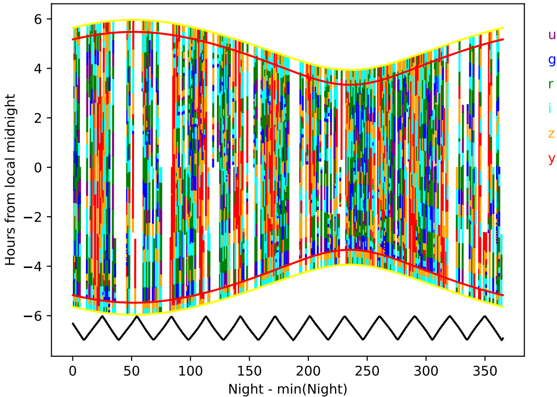
too_elab_r32_d2_gz_v3.4_10yrs year 7-8: Hourglass
