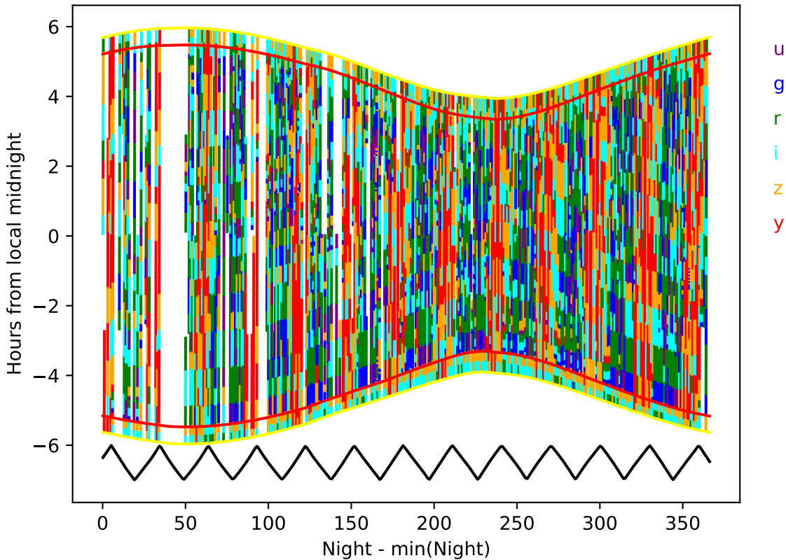
too_elab_r32_d2_gz_v3.4_10yrs year 6-7: Hourglass
