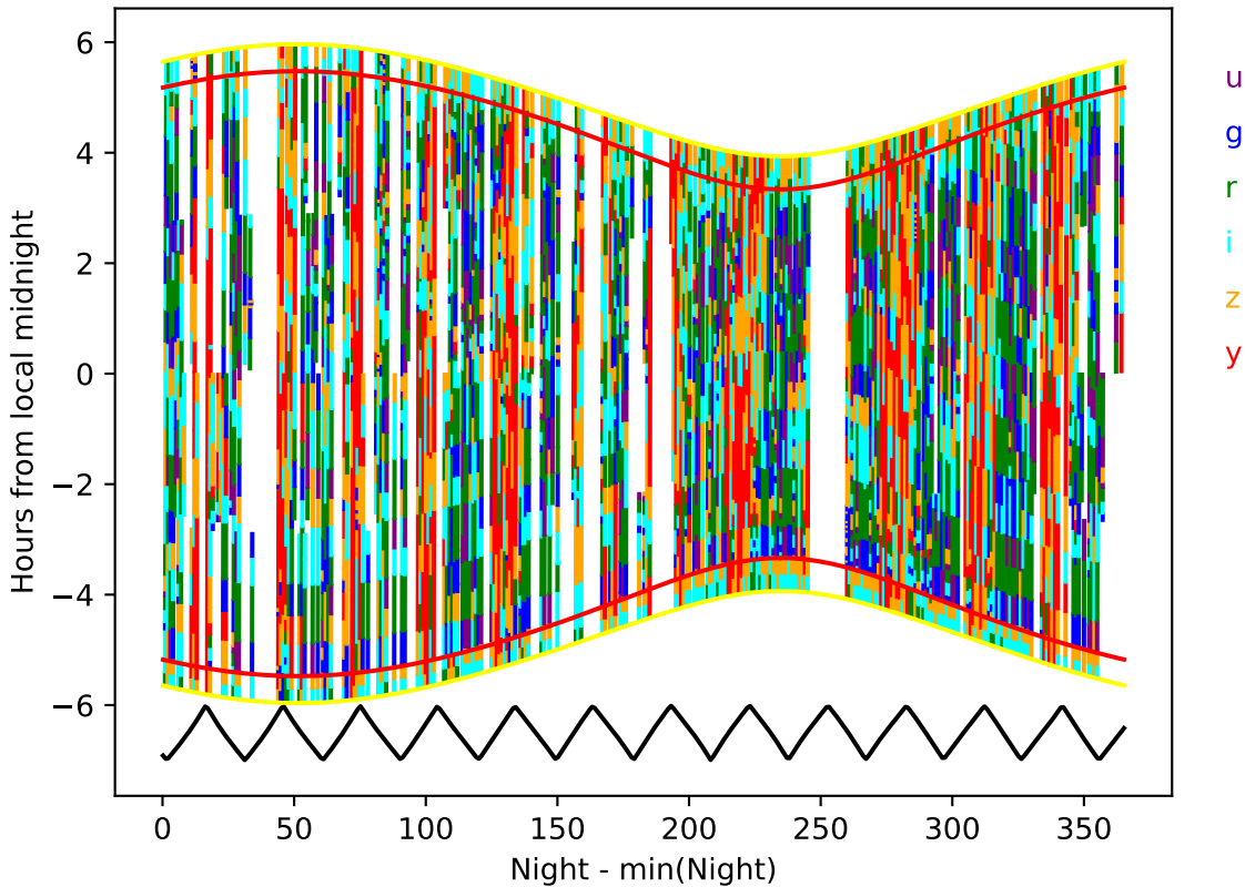
too_elab_r32_d2_gz_v3.4_10yrs year 5-6: Hourglass
