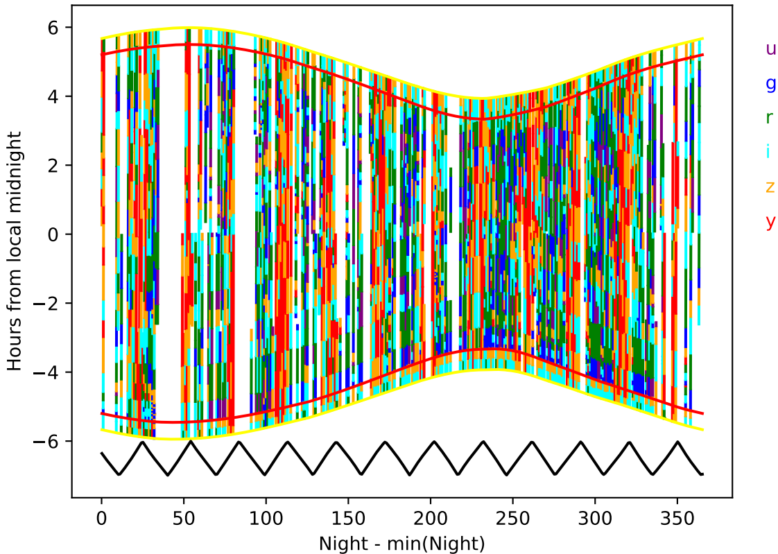
too_elab_r32_d2_gz_v3.4_10yrs year 4-5: Hourglass
