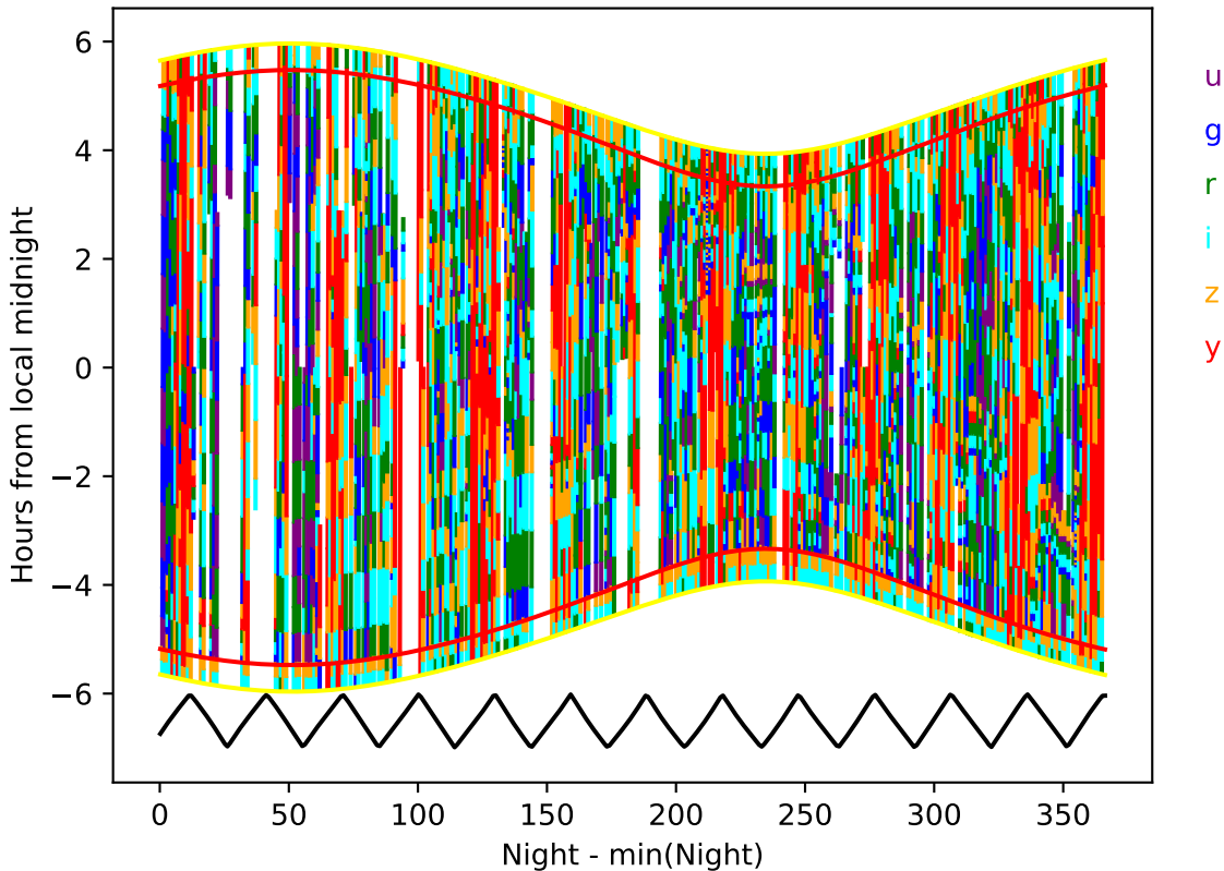
too_elab_r32_d2_gz_v3.4_10yrs year 0-1: Hourglass
