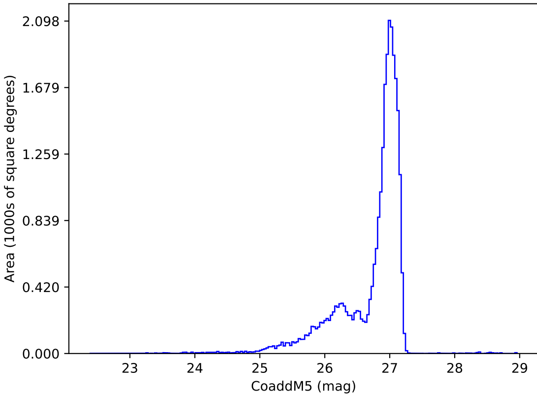
too_elab_r32_d2_gz_v3.4_10yrs r: CoaddM5
