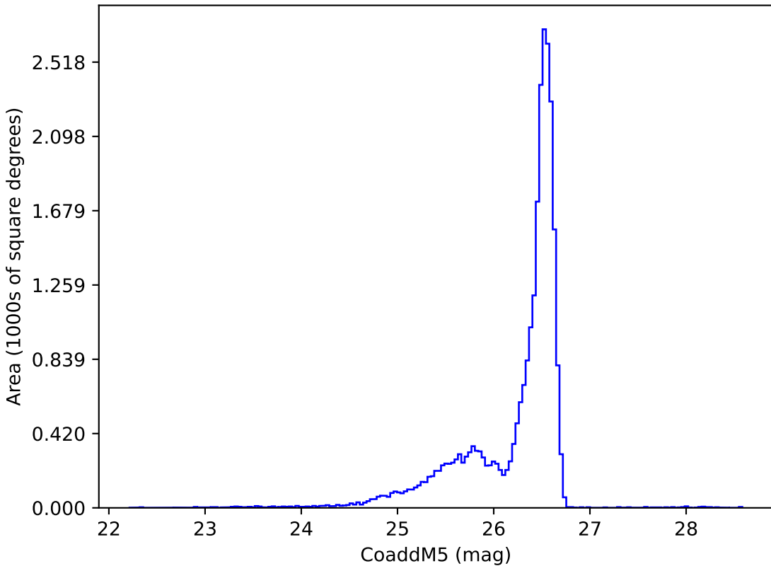
too_elab_r32_d2_gz_v3.4_10yrs i: CoaddM5
