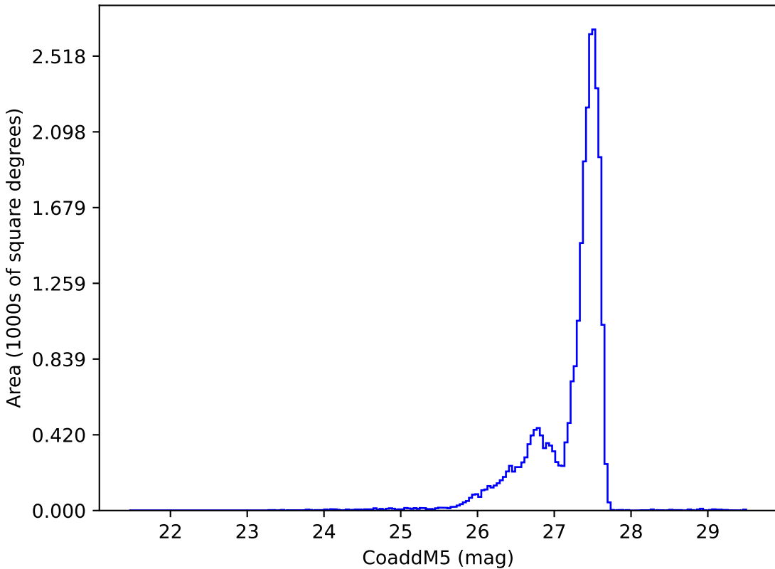
too_elab_r32_d2_gz_v3.4_10yrs : CoaddM5
