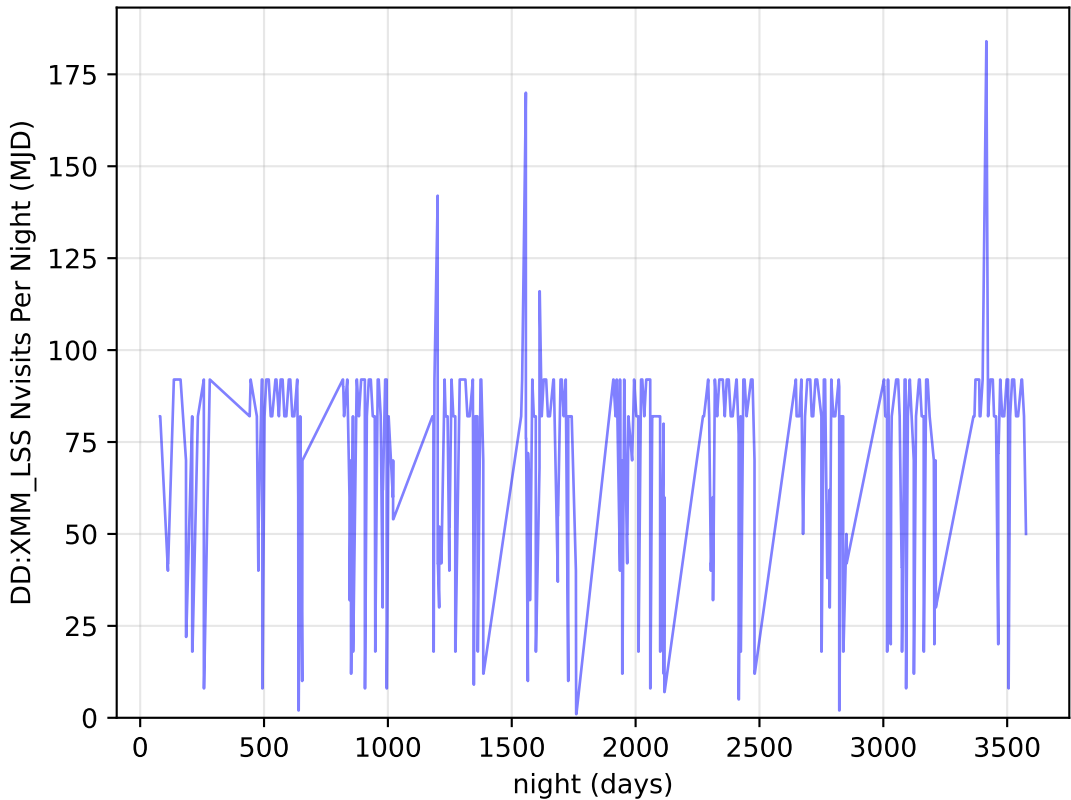
too_elab_r32_d2_gz_v3.4_10yrs all bands: DD:XMM_LSS Nvisits Per Night
