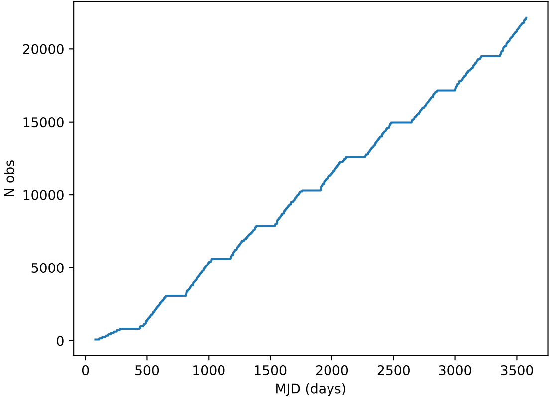
too_elab_r32_d2_gz_v3.4_10yrs all bands: DD:XMM_LSS Cumulative NVisits
