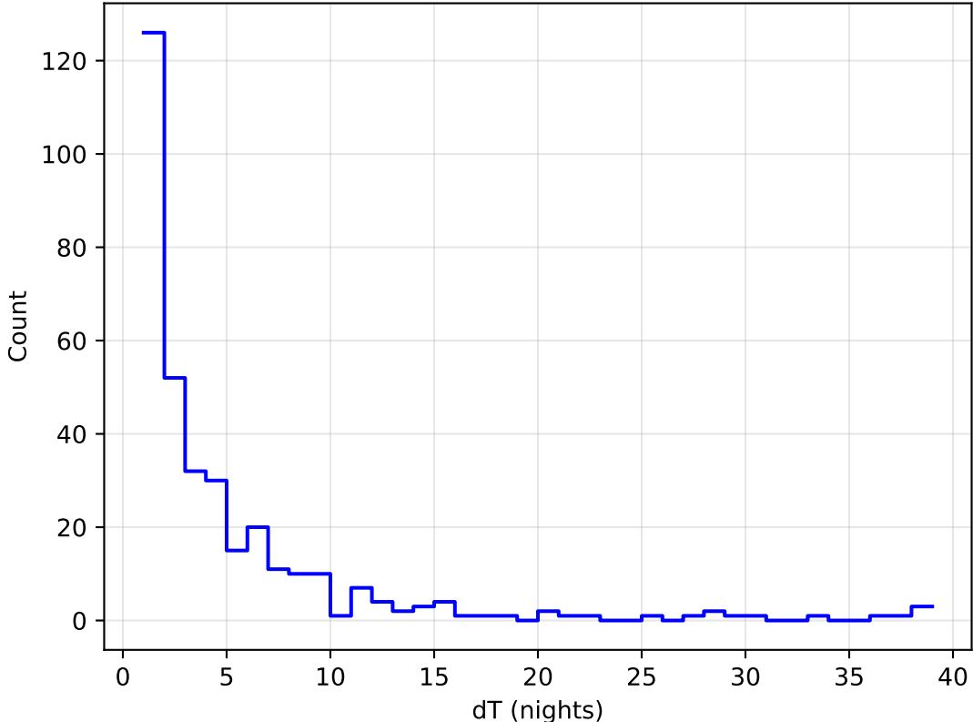
too_elab_r32_d2_gz_v3.4_10yrs all bands: DD:WFD Delta Nights Histogram
