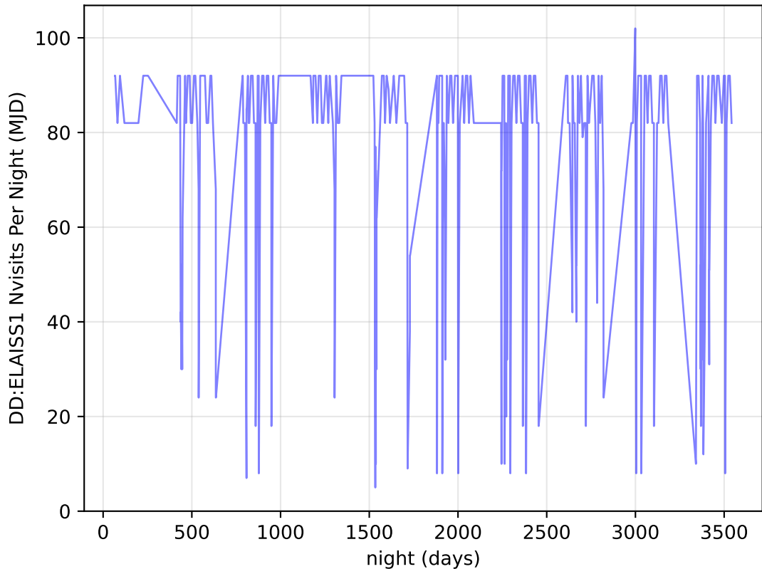
too_elab_r32_d2_gz_v3.4_10yrs all bands: DD:ELAISS1 Nvisits Per Night
