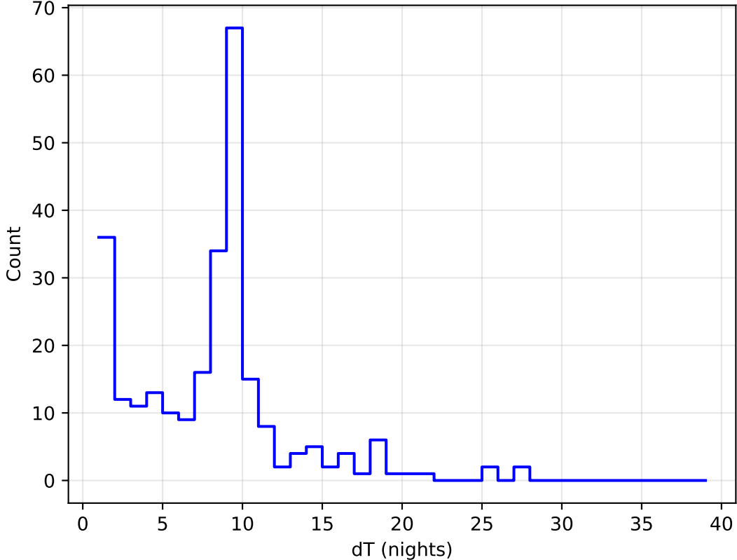
too_elab_r32_d2_gz_v3.4_10yrs all bands: DD:ELAISS1 Delta Nights Histogram
