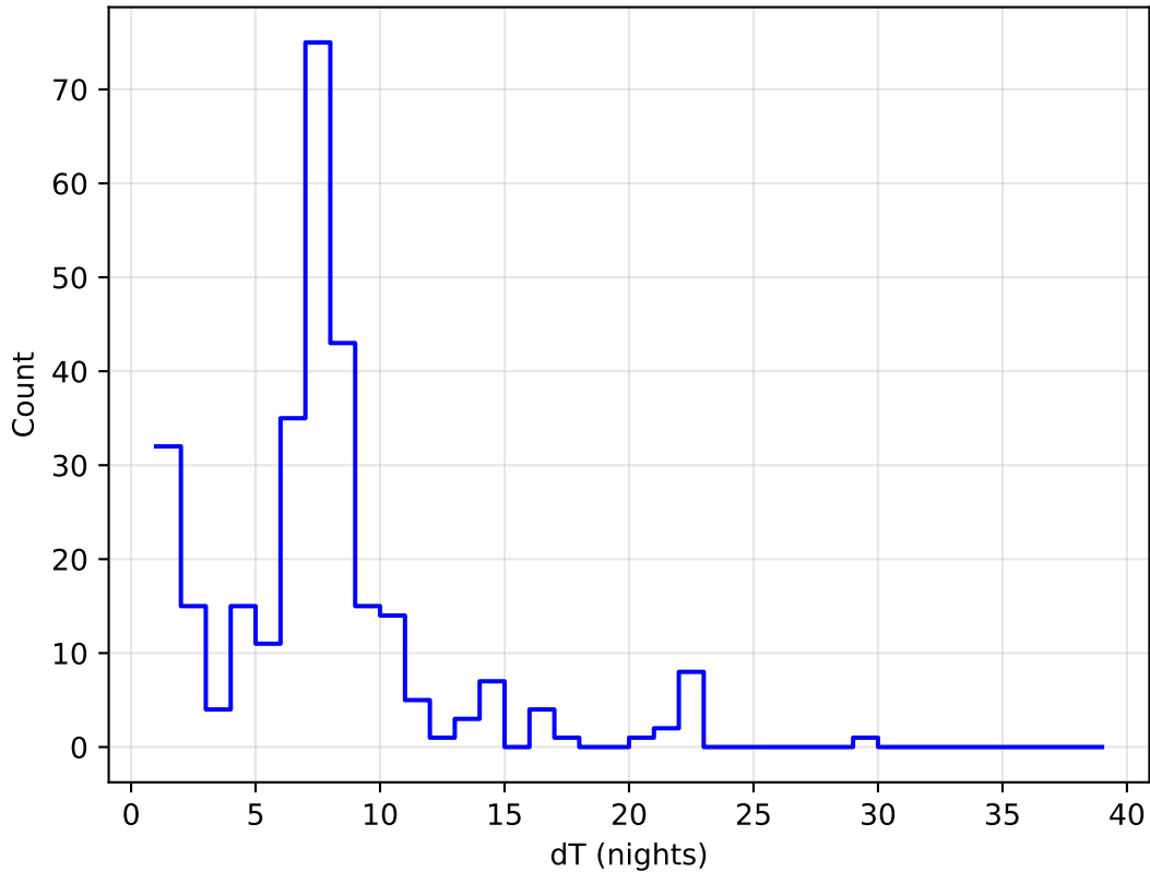
too_elab_r32_d2_gz_v3.4_10yrs all bands: DD:EDFS Delta Nights Histogram
