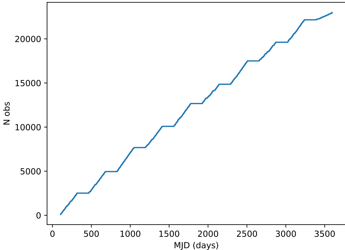
too_elab_r32_d2_gz_v3.4_10yrs all bands: DD:EDFS Cumulative NVisits
