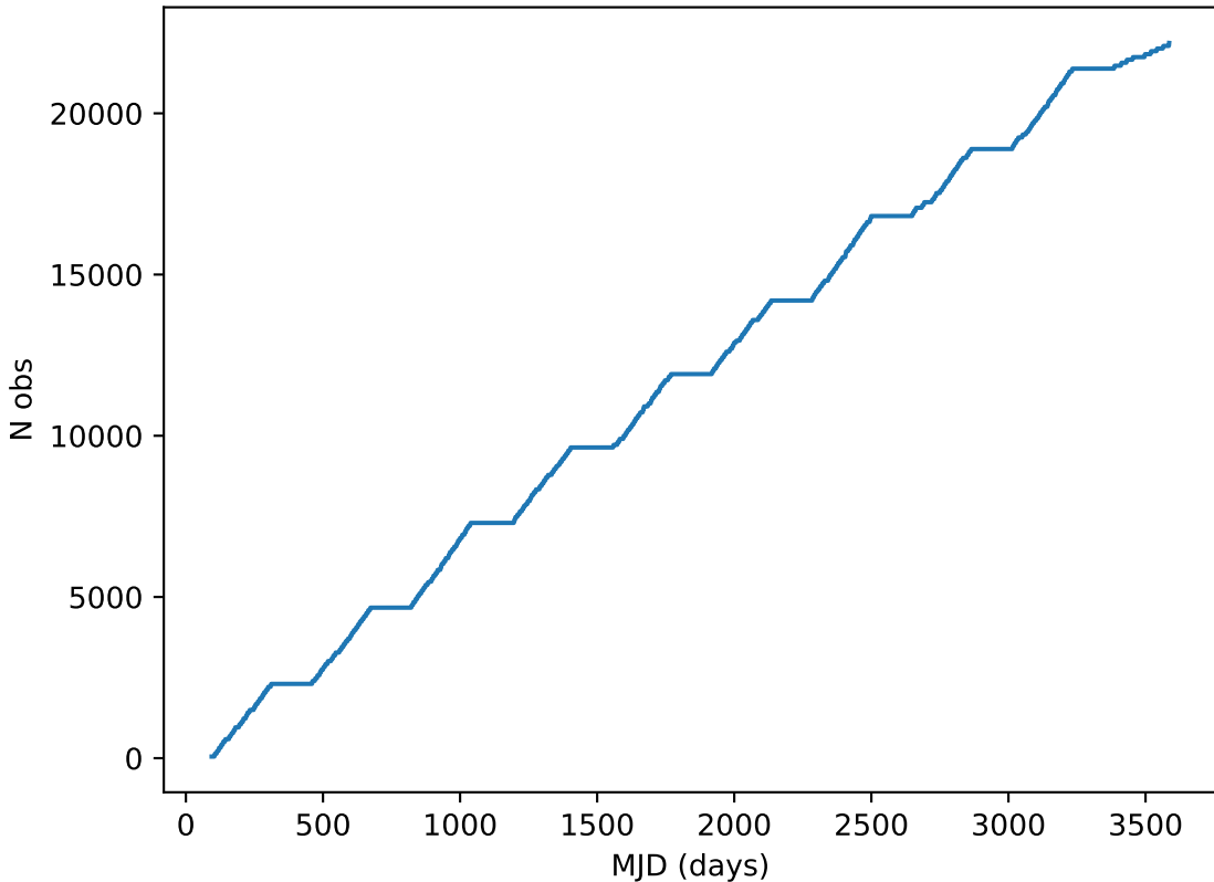
too_elab_r32_d2_gz_v3.4_10yrs all bands: DD:ECDFS Cumulative NVisits
