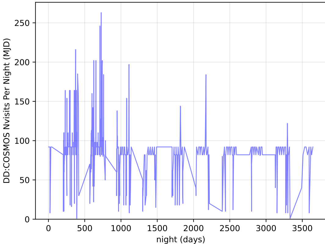
too_elab_r32_d2_gz_v3.4_10yrs all bands: DD: COSMOS Nvisits Per Night
