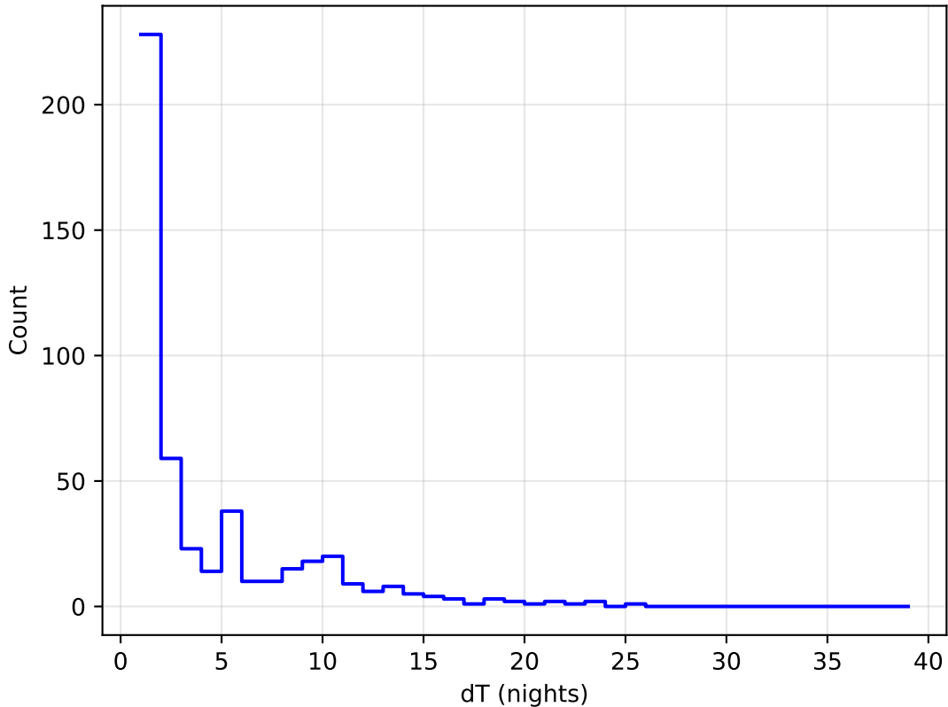
too_elab_r32_d2_gz_v3.4_10yrs all bands: DD: COSMOS Delta Nights Histogram
