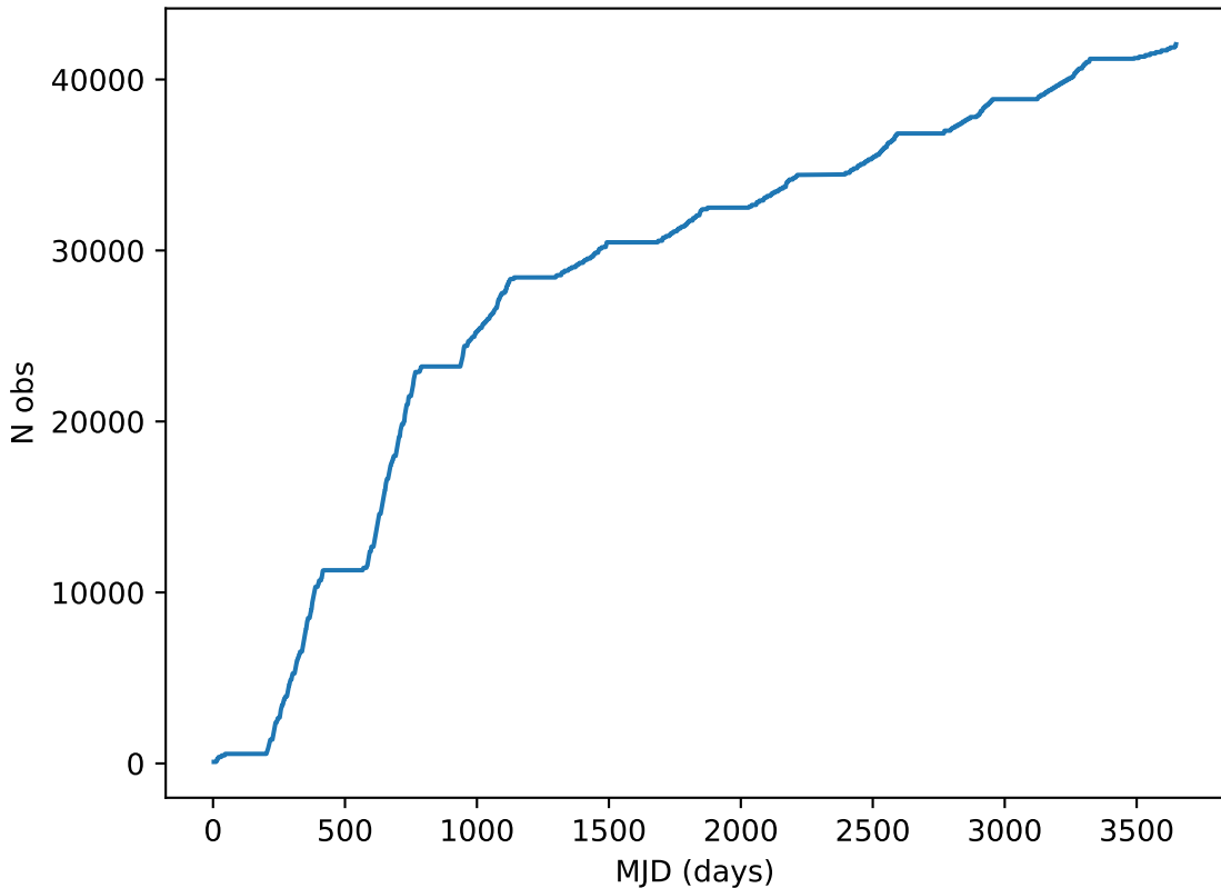
too_elab_r32_d2_gz_v3.4_10yrs all bands: DD: COSMOS Cumulative NVisits
