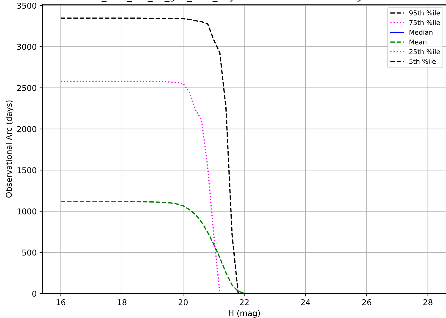
too_elab_r32_d2_griz_v3.4_10yrs: Observational Arc Length Vatira
