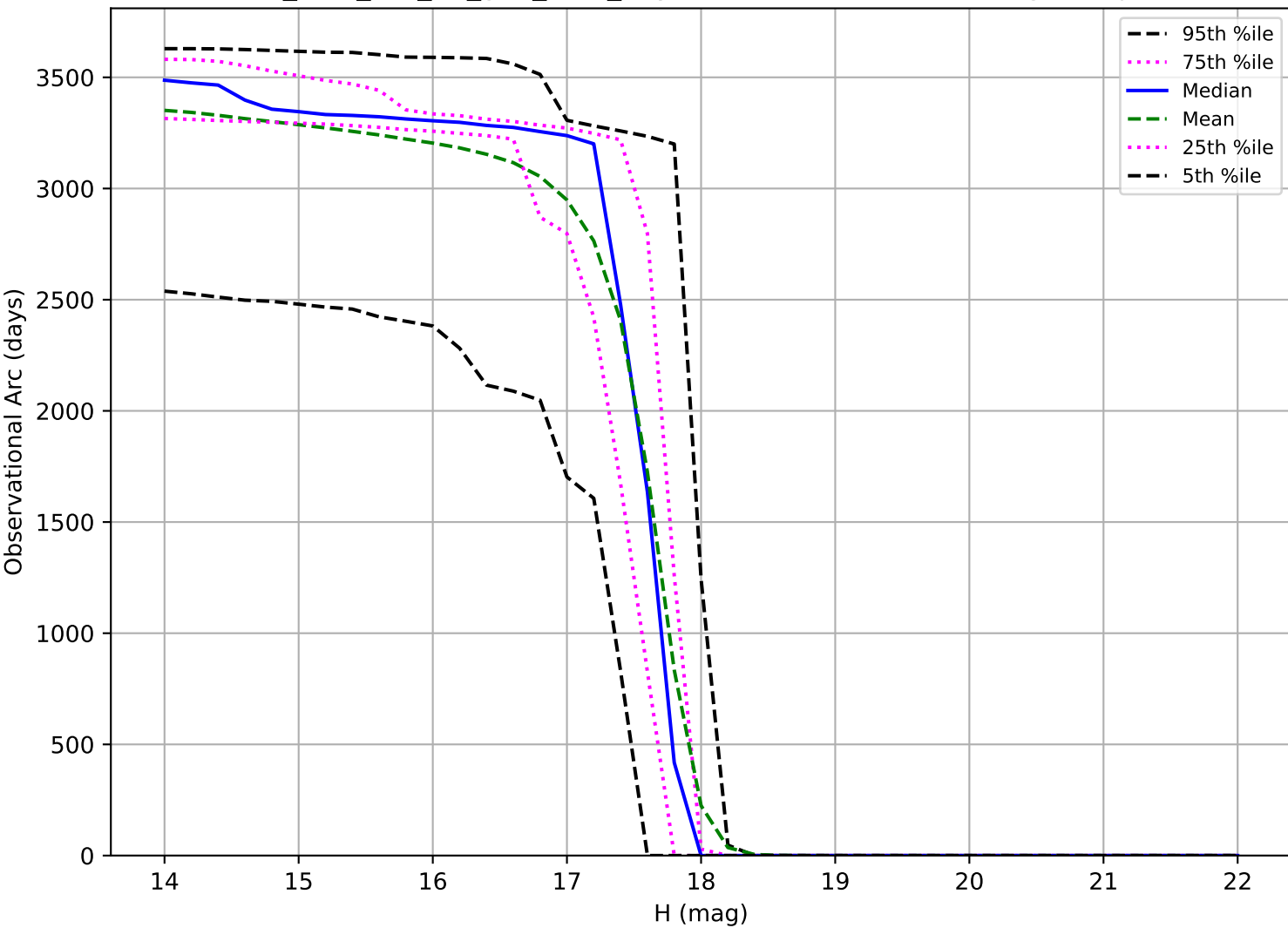
too_elab_r32_d2_griz_v3.4_10yrs: Observational Arc Length Trojan
