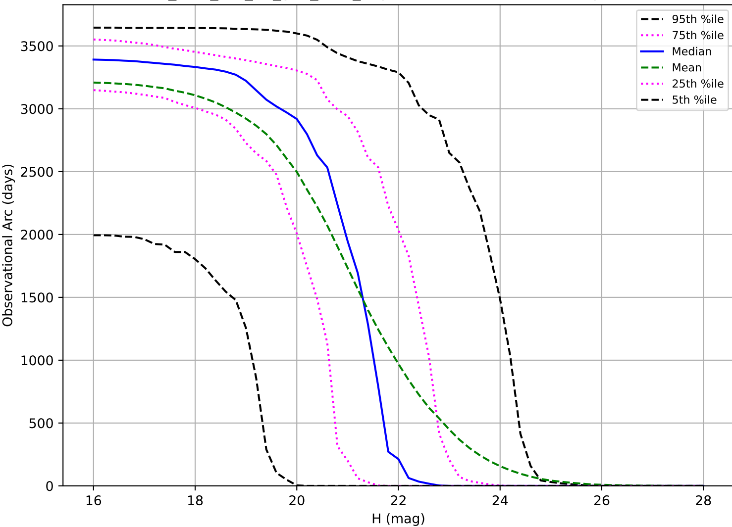
too_elab_r32_d2_griz_v3.4_10yrs: Observational Arc Length PHA
