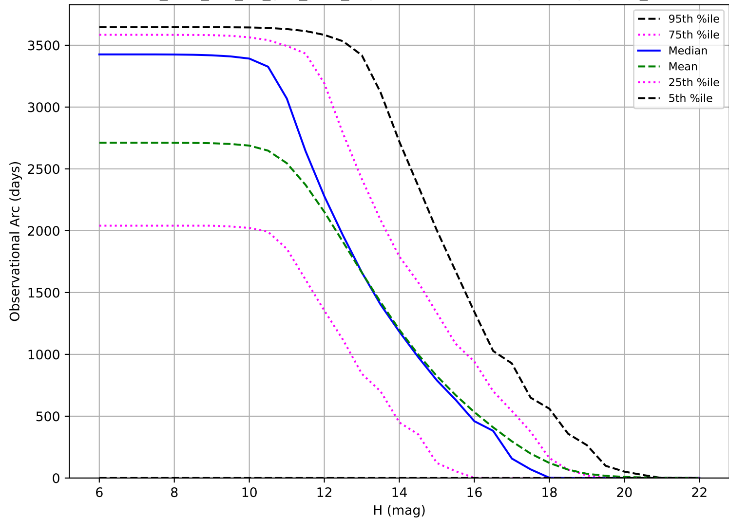
too_elab_r32_d2_griz_v3.4_10yrs: Observational Arc Length OCC_r5
