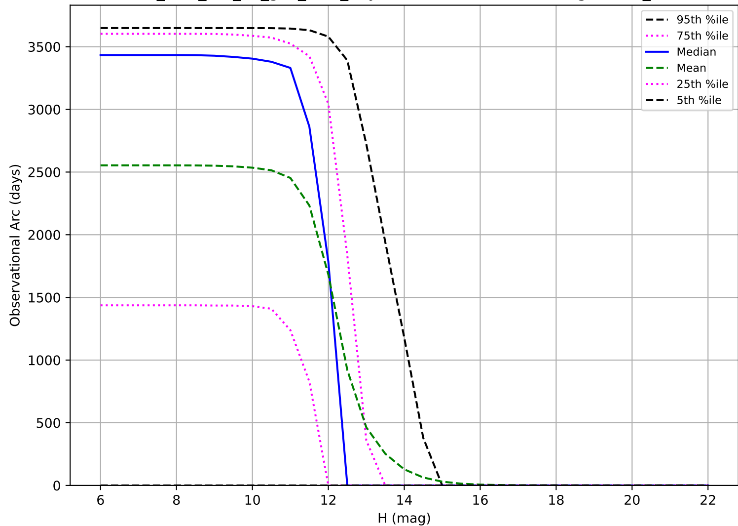
too_elab_r32_d2_griz_v3.4_10yrs: Observational Arc Length OCC_r20
