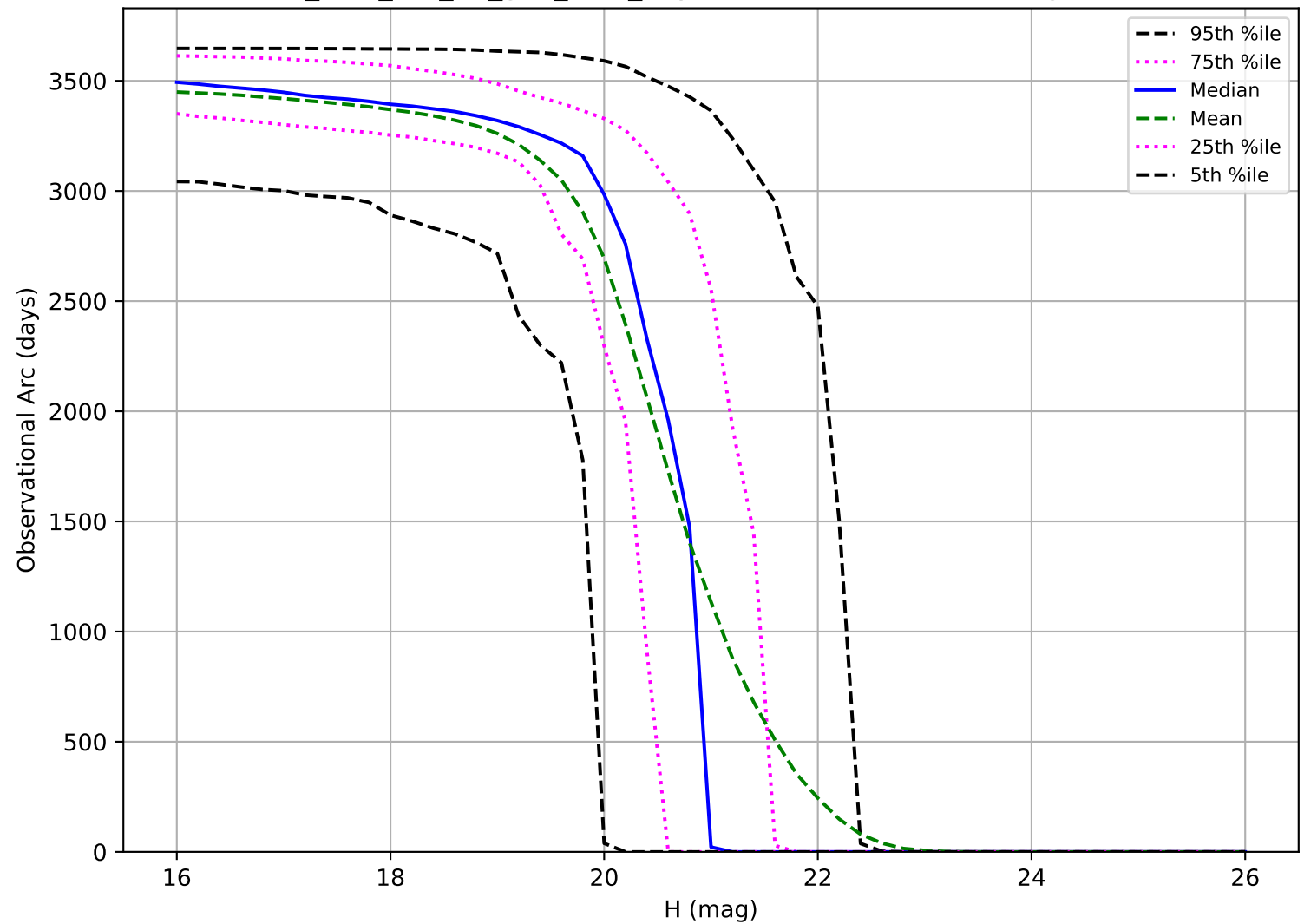
too_elab_r32_d2_griz_v3.4_10yrs: Observational Arc Length MBA
