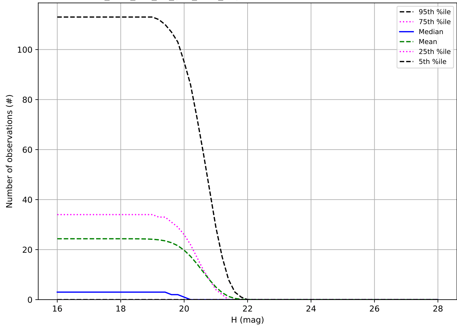
too_elab_r32_d2_griz_v3.4_10yrs: Number of observations Vatira
