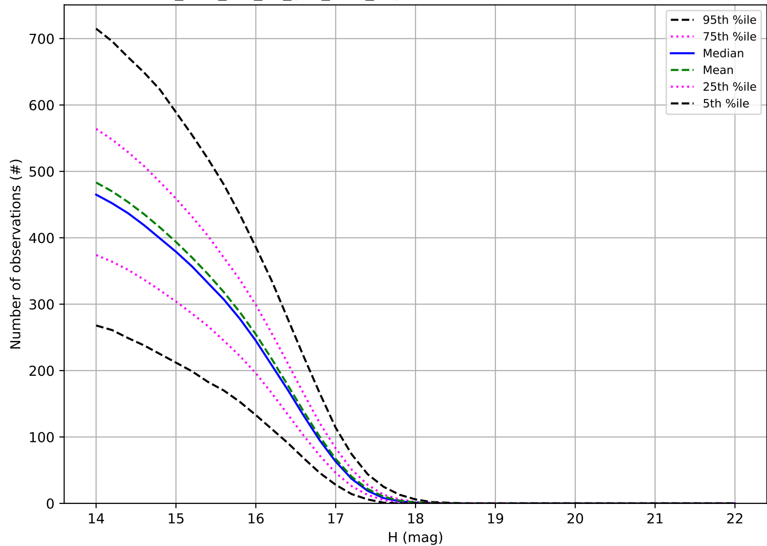
too_elab_r32_d2_griz_v3.4_10yrs: Number of observations Trojan
