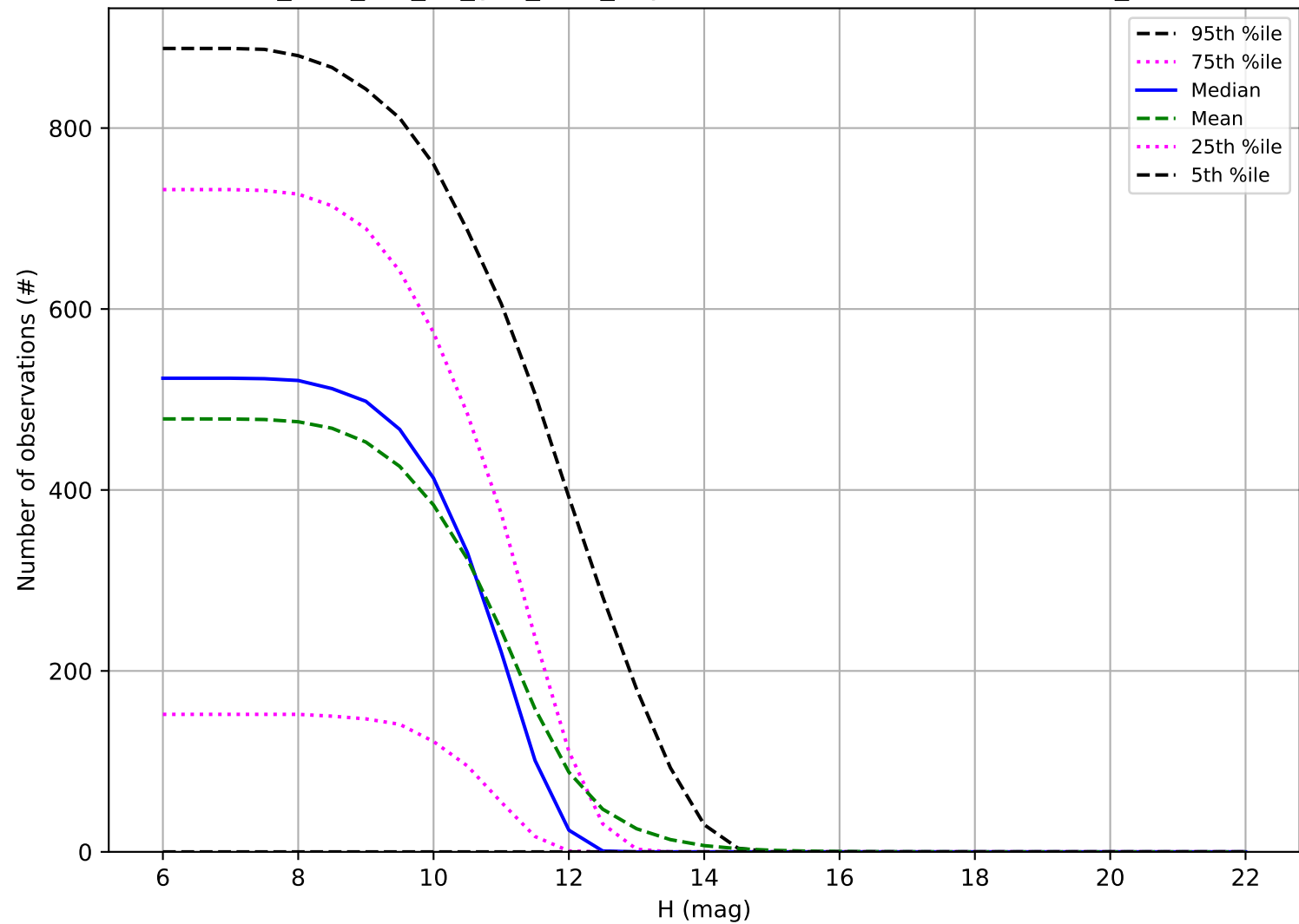
too_elab_r32_d2_griz_v3.4_10yrs: Number of observations OCC_r20
