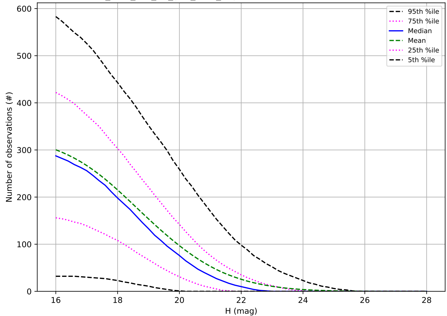
too_elab_r32_d2_griz_v3.4_10yrs: Number of observations NEO
