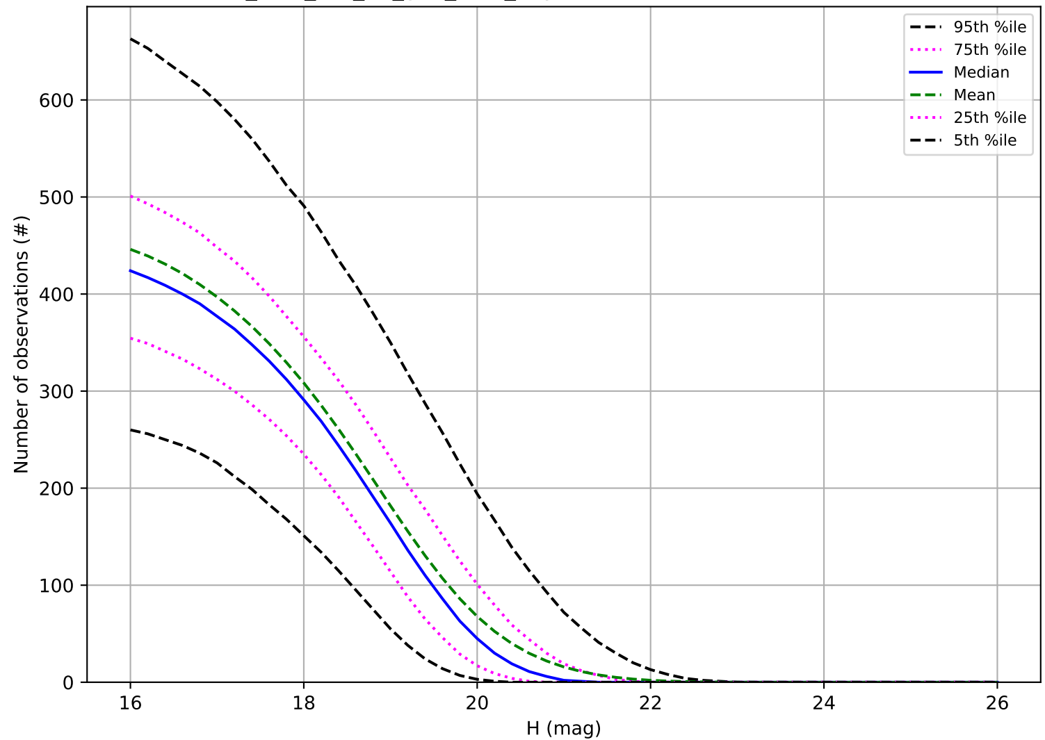
too_elab_r32_d2_griz_v3.4_10yrs: Number of observations MBA
