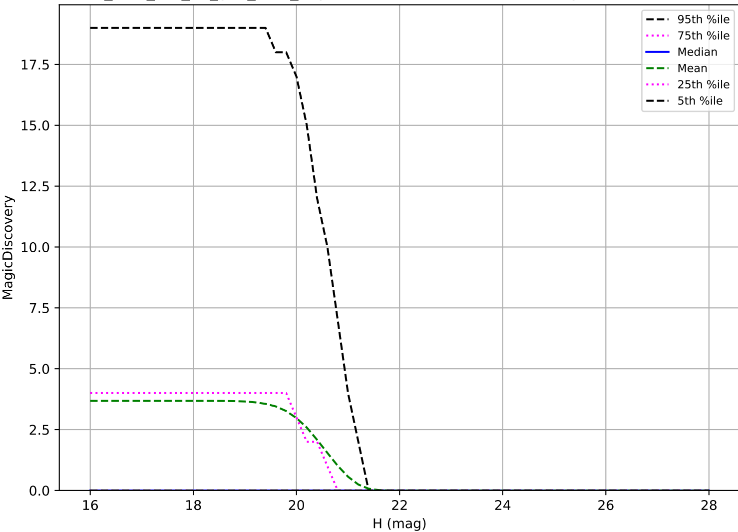
too_elab_r32_d2_griz_v3.4_10yrs: Vatira 6 detections in 60 nights detection loss
