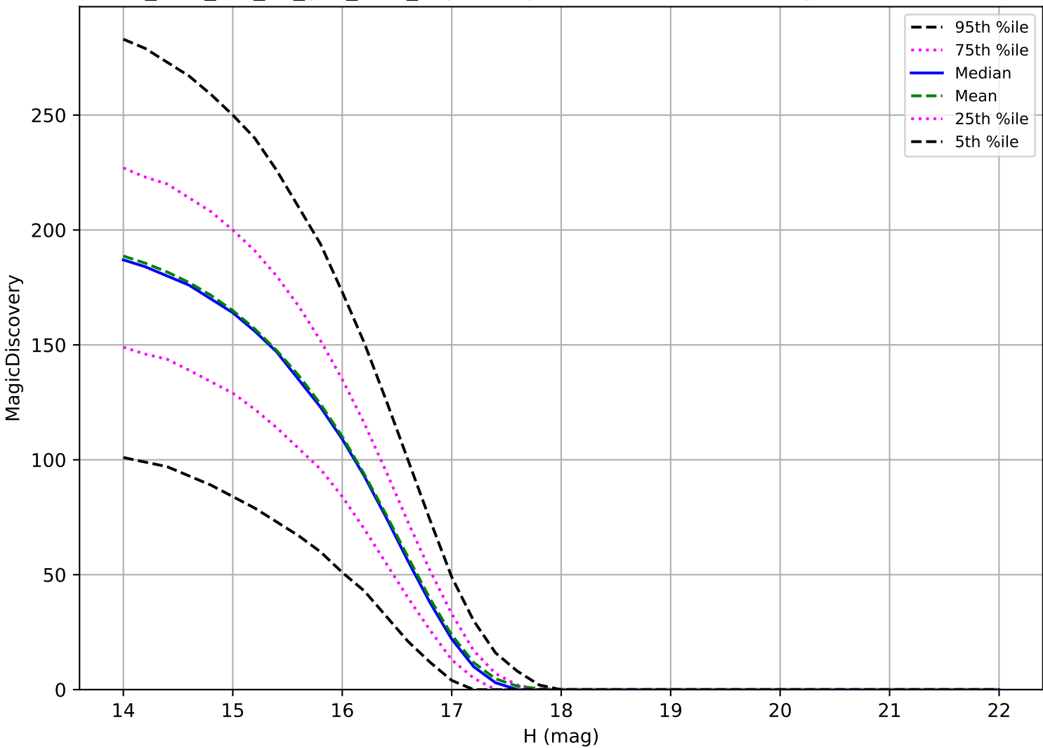
too_elab_r32_d2_griz_v3.4_10yrs: Trojan 6 detections in 60 nights detection loss
