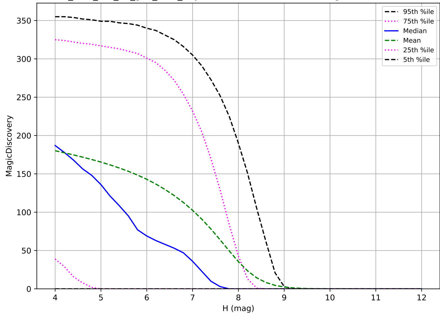
too_elab_r32_d2_griz_v3.4_10yrs: TNO 6 detections in 60 nights detection loss
