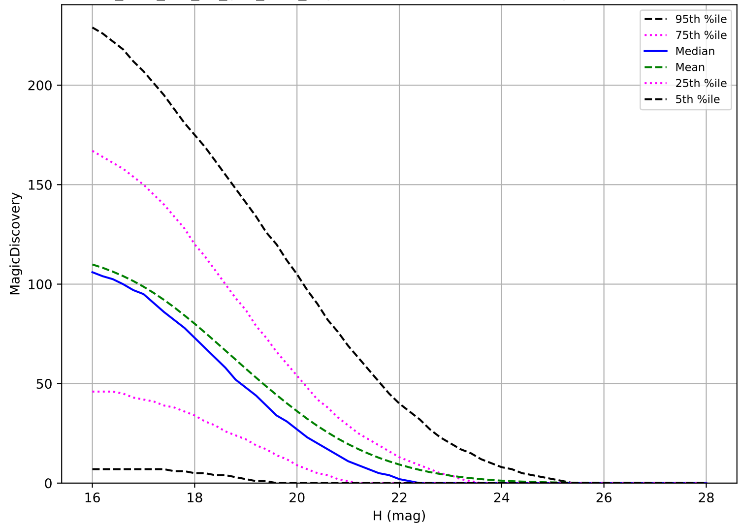
too_elab_r32_d2_griz_v3.4_10yrs: PHA 6 detections in 60 nights detection loss
