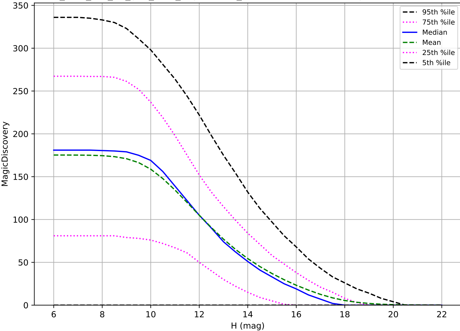
too_elab_r32_d2_griz_v3.4_10yrs: OCC_r5 6 detections in 60 nights detection loss
